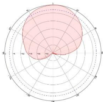
1710-2170 Horizontal pattern
