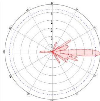
1710-2170 Vertical pattern
